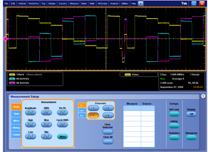
Oscilloscope Measurement Menu.
